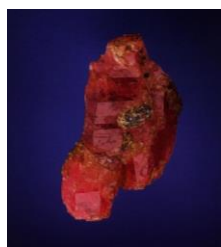
Fig.4A: Ruby from Dhadhing
