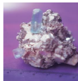
Fig.4C: Aquamarine from Taplejung
