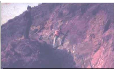
Fig.2B: Bamangaon polymetallic deposit
